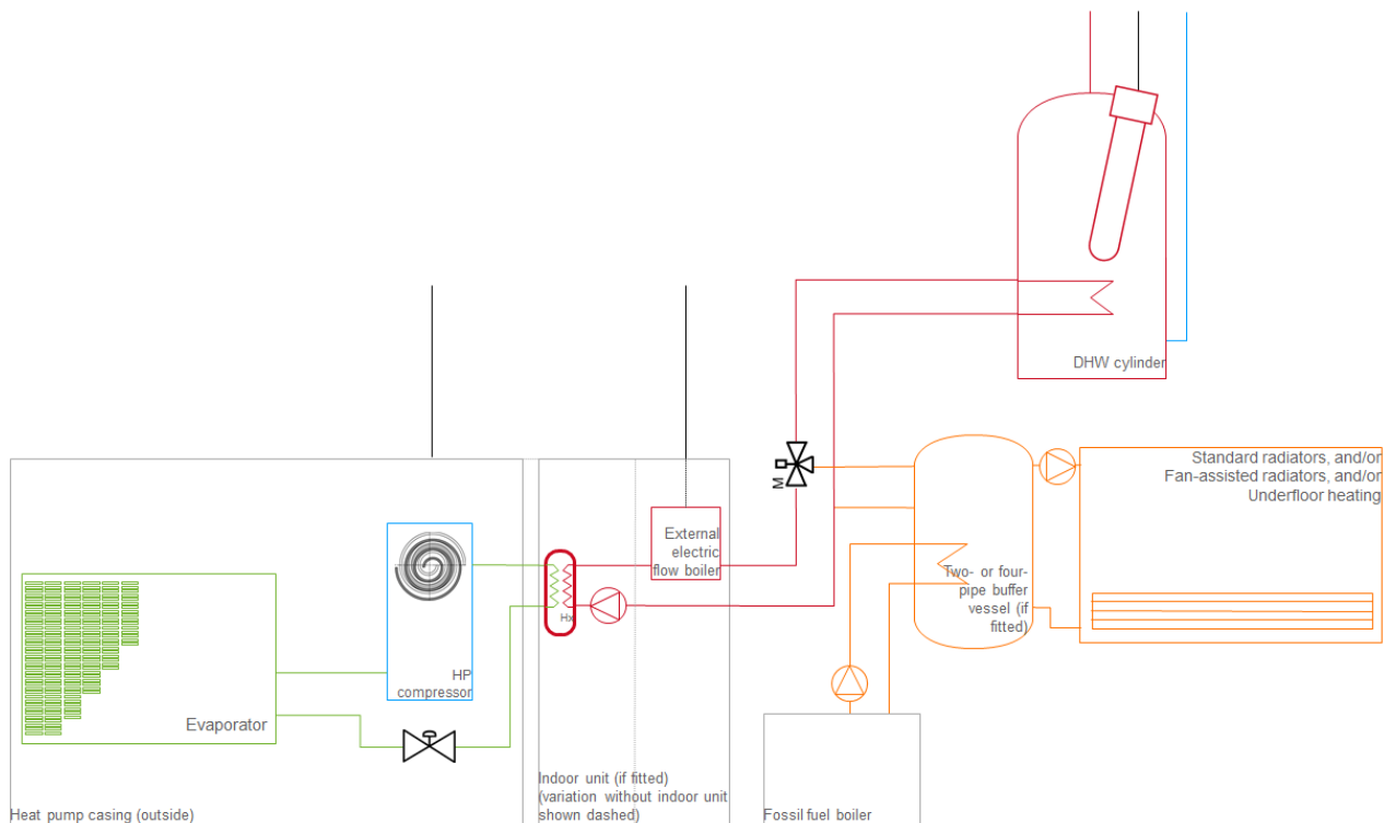
Figure 24: Worked Example 3 – Split-system ASHP with back-up fossil fuel boiler and an immersion element in the domestic hot water cylinder
