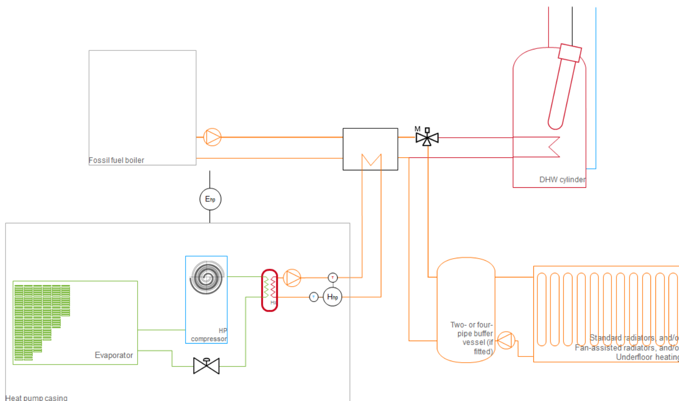
Figure 10: Air-source heat pump with back-up fossil fuel boiler showing metering option 2: 1 heat meter (integrated) and 1 electricity meter
