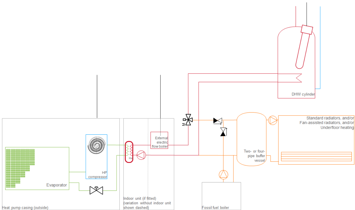
Figure 14: Split-system air-source heat pump providing space heating and hot water
